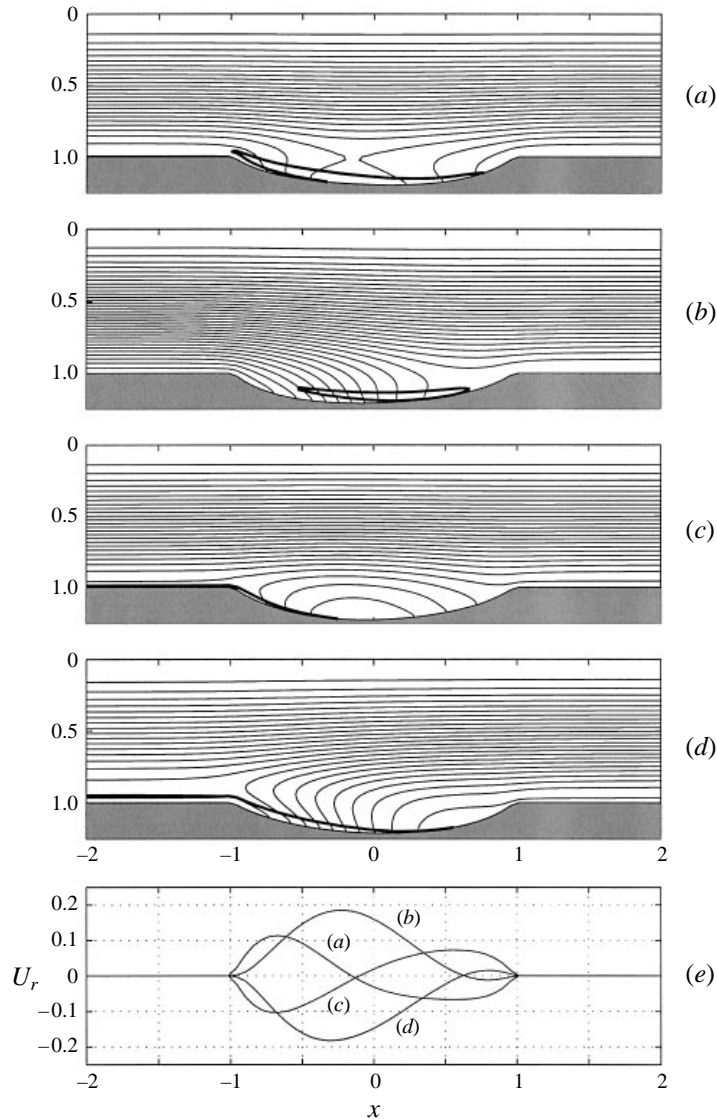
FIGURE 8. Oscillatory flow for K = 50 , C = 10 , p_{ref} = 10 and unsteady forcing \varepsilon = 10^{-2} , S_t = 0.65^{-1} . Instantaneous streamlines at (a) 0/4, (b) 1/4, (c) 2/4, (d) 3/4 of the period of upstream flow oscillation, streamfunction levels from 0 to 0.7, step 0.02, the thick lines corresponds to the zero vorticity contour. (e) Corresponding membrane radial velocity.
